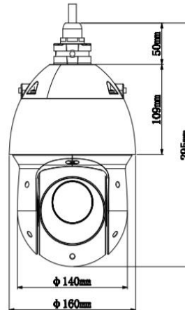
Dimensions (mm)
